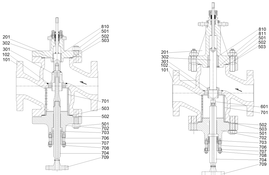
MV 5351, PV 6351 DN 40 – 150, PN 16 – 40
